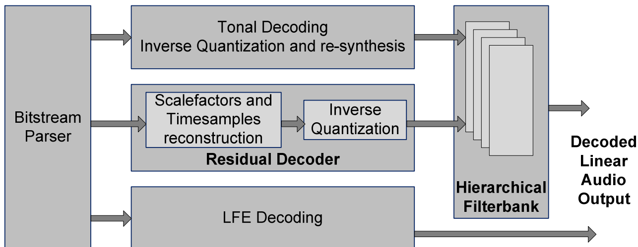
Figure 9-4: LBR Decoder Overview
