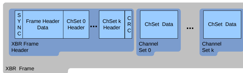
Figure 6-9: XBR Data Frame Structure
