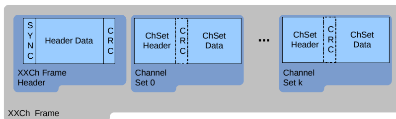
Figure 6-11: XXCH Data Frame Structure
